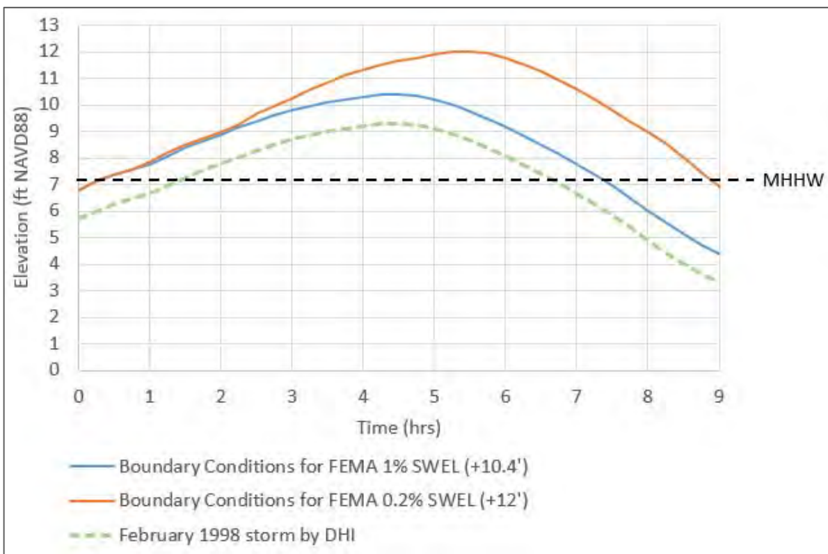
Figure 3-4: Boundary Conditions Developed for Unsteady Modeling
